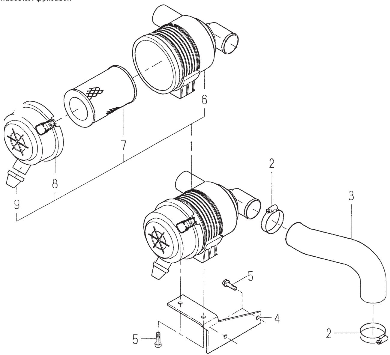
673 AIR CLEANER
